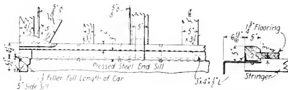
Fig. 3—Grain Tight End Sill for Steel Underframe Cars
